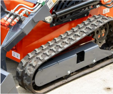
Rubber tracks and lift arm
